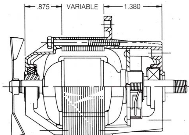
Totally enclosed or skeleton motors
